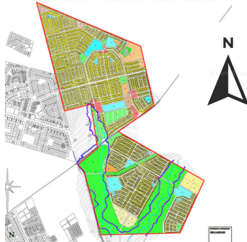
PROPOSED TOWNSHIP LAYOUT PLAN: HILLVIEW
